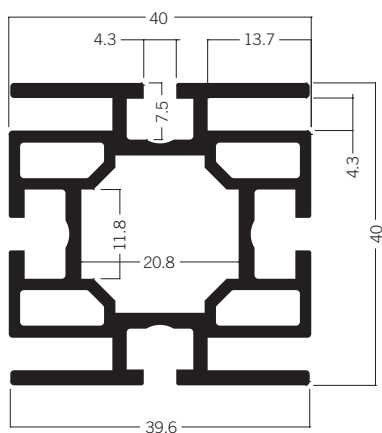
M 1305 Tension fabric extrusion 40 mm 8.23 kg
