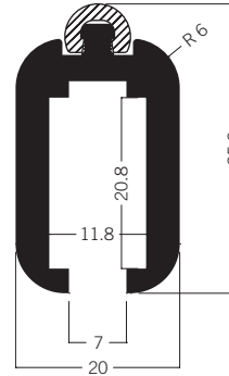
E 800 Wardrobe rail extrusion 4.30 kg
