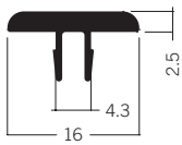
E 458 Cover extrusion 0.38 kg
