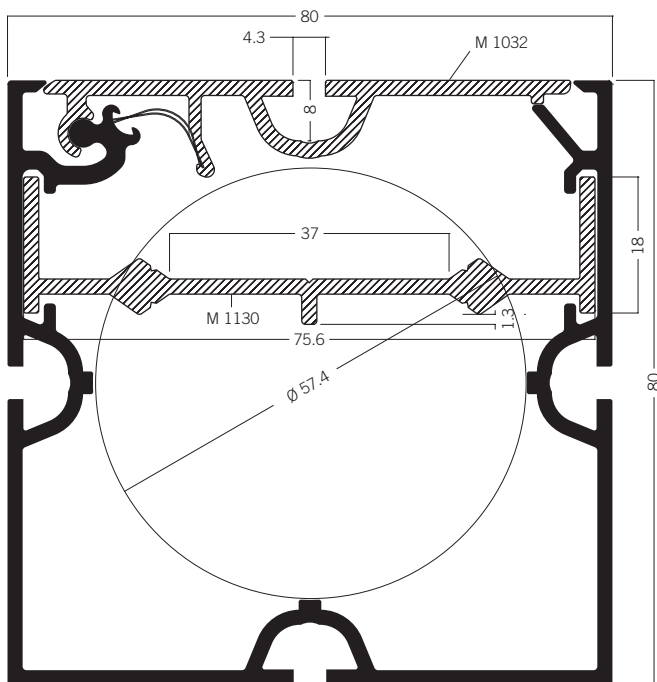
M 1022** Square extrusion 80mm 15.66 kg
