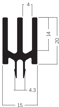
M 1319 Tension fabric extrusion 20 mm 1.46 kg
