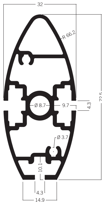
S 6105* Oval extrusion 32 × 72.5 mm 7.65 kg
