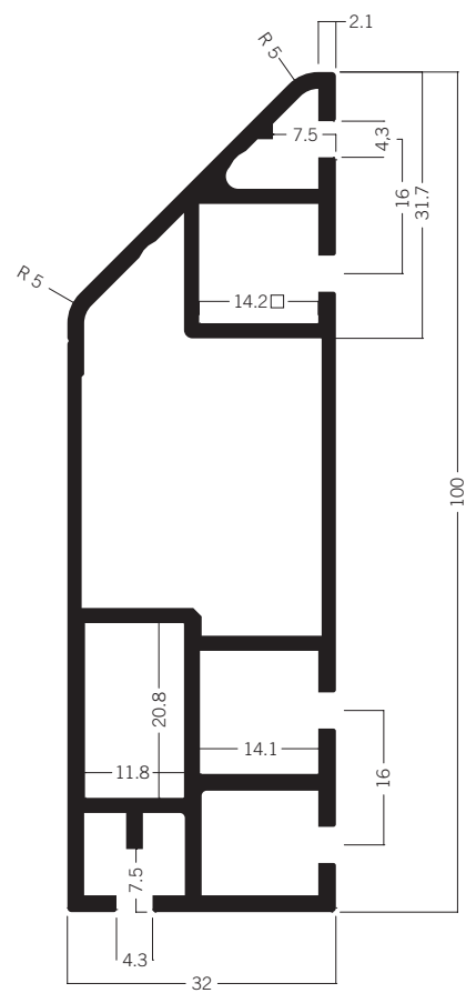
S 1310* Triangular extrusion 100 mm 9.28 kg
