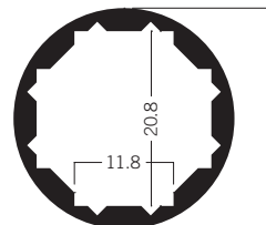
M 1208 Round extrusion 26.3 mm 2.17 kg
