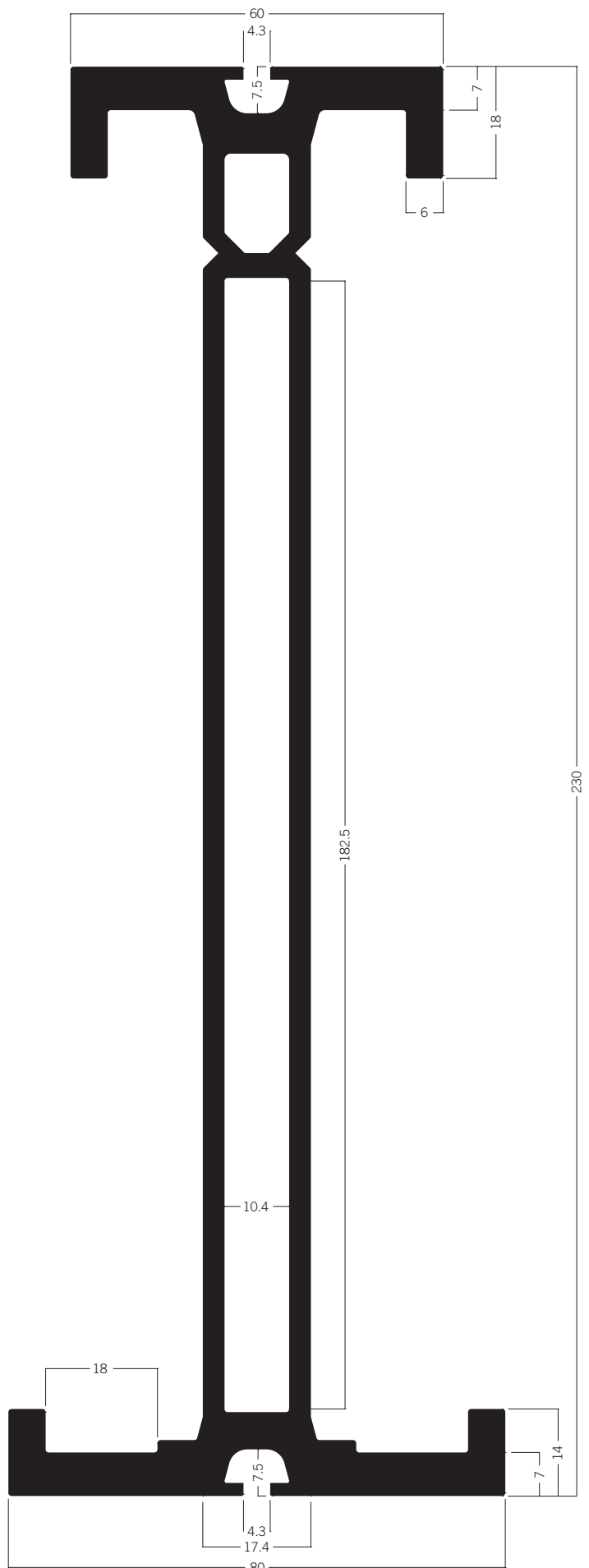
DFL 230 Beam extrusion 230 mm 53.24 kg
