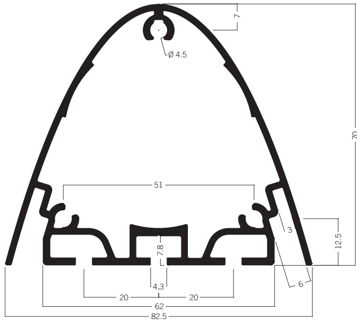
S 3050 * Oval extrusion 11.34 kg
