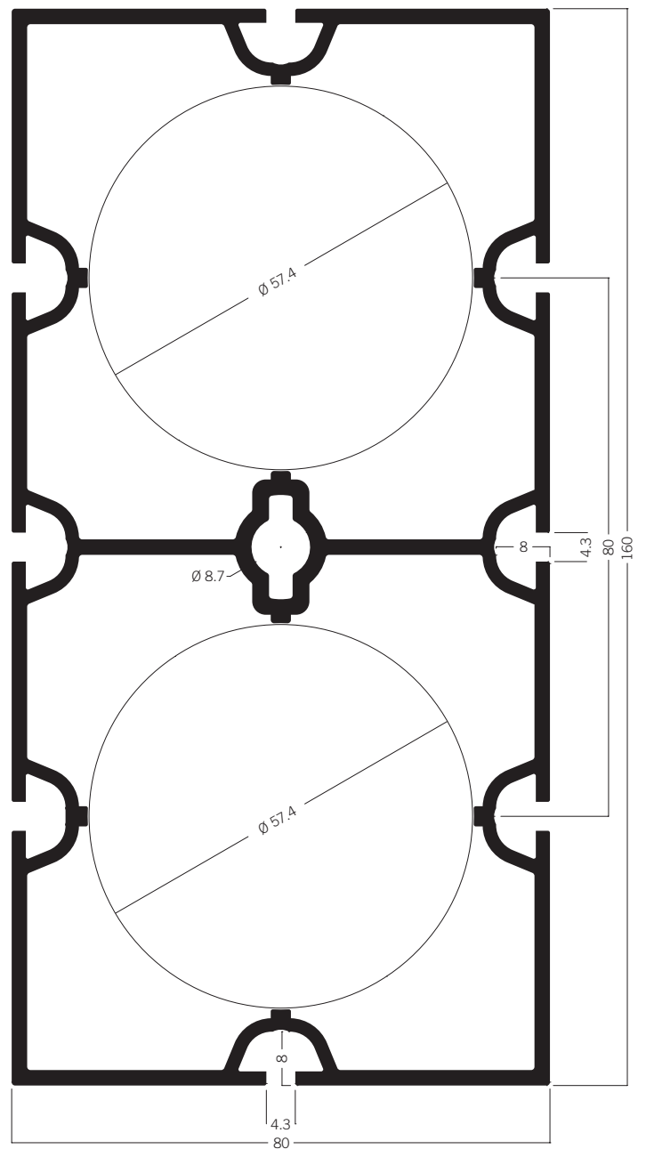
M 1052 * Rectangular extrusion 160 mm 28.35 kg
