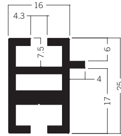
M 1603** Beam extrusion 25 mm 2.74 kg
