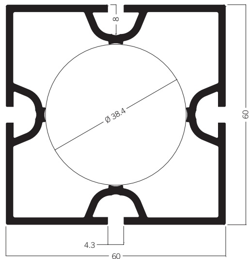
M 1010* Square extrusion 60 mm 8.13 kg
