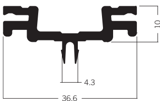
C 160* Adaptor extrusion 10 × 37 mm 1.61 kg
