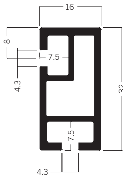
Z 307* Beam extrusion 32 mm 2.53 kg
