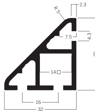
S 1303* Triangular extrusion 32 mm 3.19 kg
