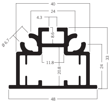
S 1610** Frame extrusion 48 mm 6.48 kg
