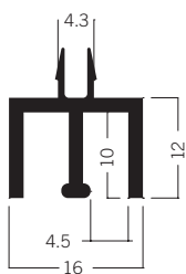
E 400 Upper track for sliding doors 0.60 kg
