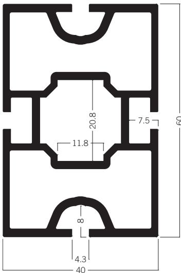
M 1081 * Rectangular extrusion 60 mm 8.94 kg
