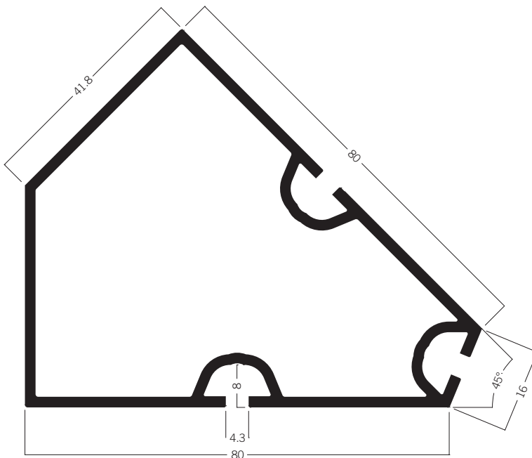
M 1070 Exterior corner extrusion 135° 8.38 kg
