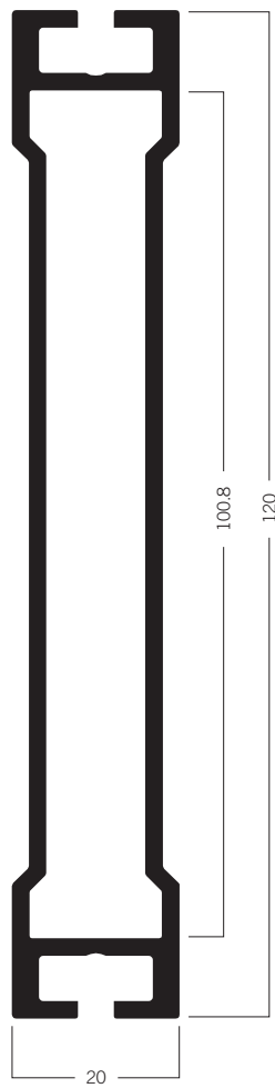
U 1030** Beam extrusion 120 mm 9.51 kg
