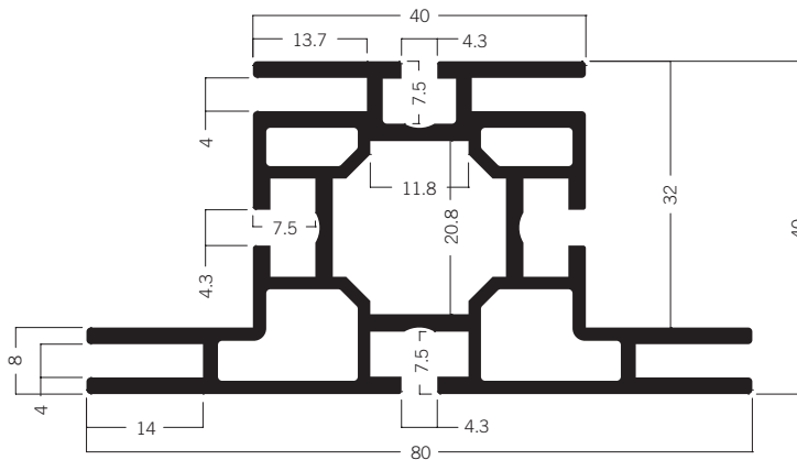
M 1304* Tension fabric extrusion 80 mm 10.15 kg
