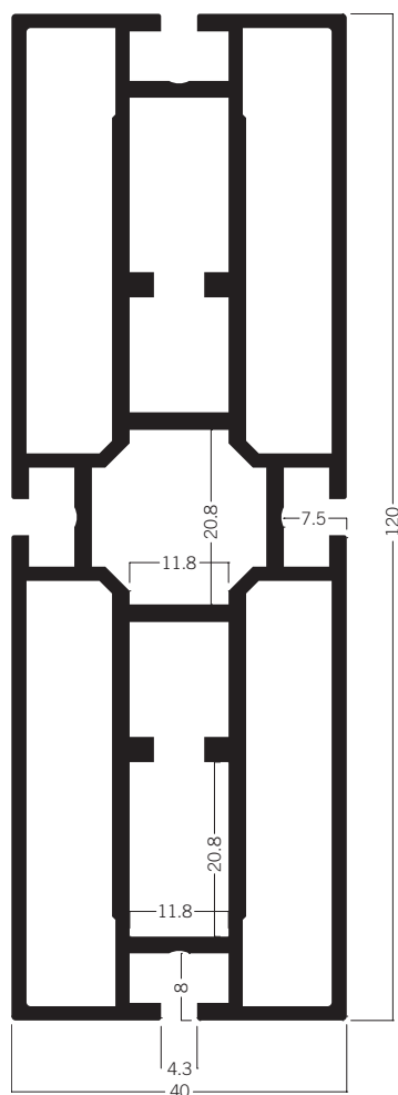
M 1031 Rectangular extrusion 120 mm 18.07 kg
