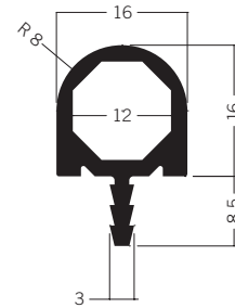
S 252* Hinged extrusion 16 mm 1.73 kg
