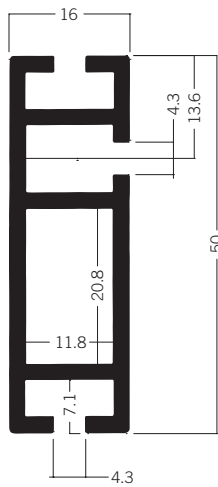
Z 464* Beam extrusion 50 mm 4.11 kg
