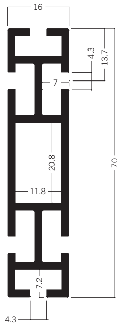
Z 160* Beam extrusion 70 mm 5.43 kg
