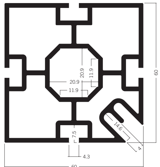
S 385R* upright extrusion, with silicone edge groove (USA)
