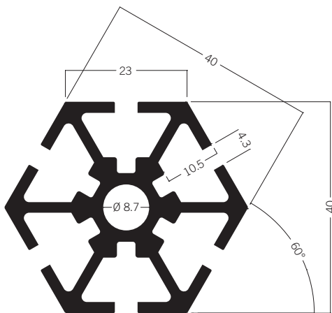
S 500 Upright extrusion 60° 6.98 kg
