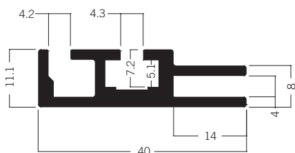
M 1930 Tension fabric extrusion for light frame 40 mm 3.41 kg
