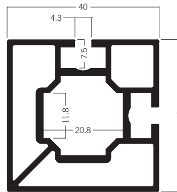
M 1007 Square extrusion 40 mm 7.17 kg
