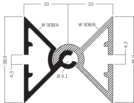
W 908 Hinged extrusion 5.60 kg
