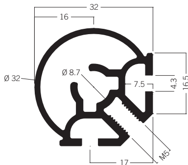
S 1200* Quarter-round extrusion 3.78 kg
