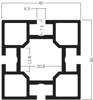
M 1000 Square extrusion 40 mm 5.78 kg
