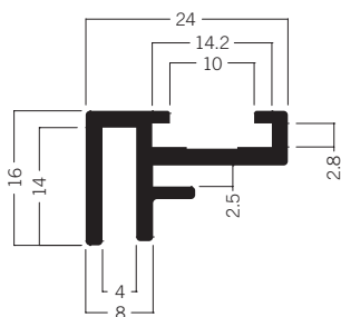
M 1607 Tension fabric extrusion 16 mm 1.91 kg
