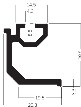
M 1326* Connection extrusion, cube 3.27 kg
