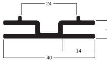
M 1310 Tension fabric extrusion 40 mm 2.69 kg
