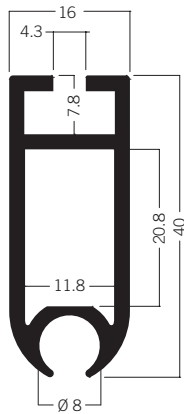
M 1354 Fabric suspension extrusion 40 mm 3.18 kg
