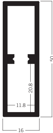
Z 402 Beam extrusion 50 mm 3.76 kg
