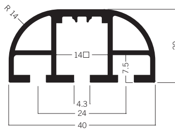
M 1606* Semi-circular extrusion 3.04 kg
