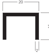
M 1312* U-channel extrusion 1.56 kg
