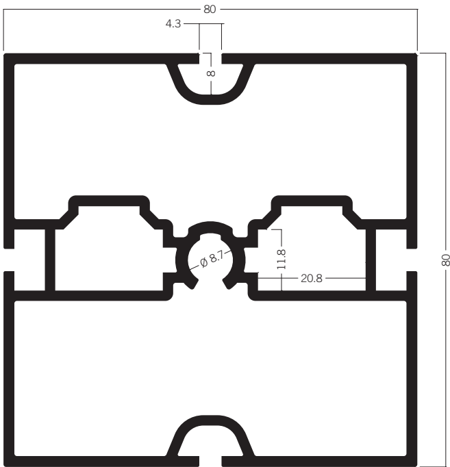
M 1018 Square extrusion 80 mm 14.91 kg
