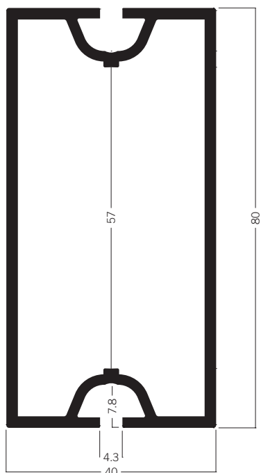
M 1043* Rectangular extrusion 80 mm
