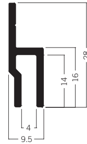
M 1614 Tension fabric extrusion 28 mm 1.54 kg
