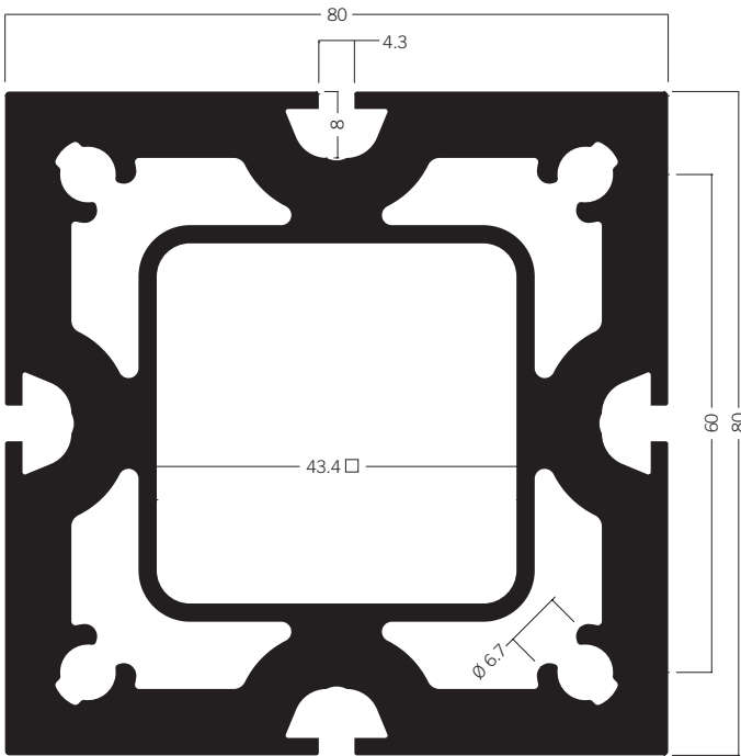
DFS 84 Upright extrusion 80 mm 38.95 kg
