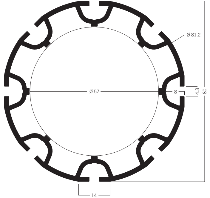
M 1222* Round extrusion 80 mm 10.97 kg
