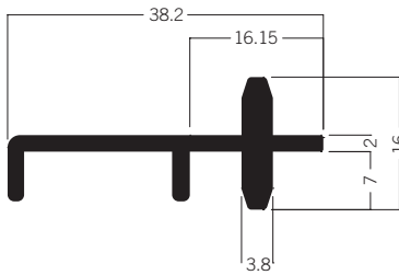
M 1567 Wall panel retainer, center 2.04 kg
