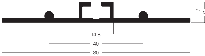
WP 830* Cover extrusion
