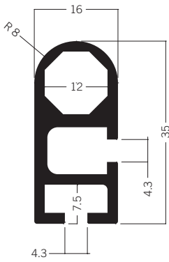
S 250 Hinged extrusion 35 mm 3.14 kg
