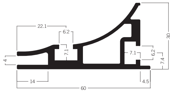
M 1920* Tension fabric extrusion for light frame 60 mm 6.07 kg
