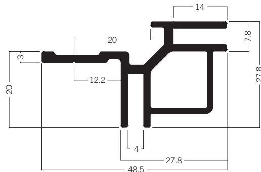
M 1322/E * Tension fabric extrusion, external corner 4.42 kg
