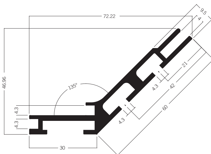
M 1301 Tension fabric extrusion 135° 6.55 kg
