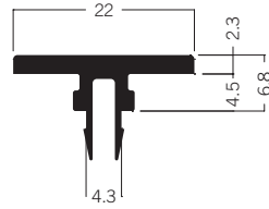
M 1844* Cover extrusion 0.42 kg
