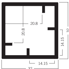
S 1123* Square extrusion 32 mm 3.77 kg
