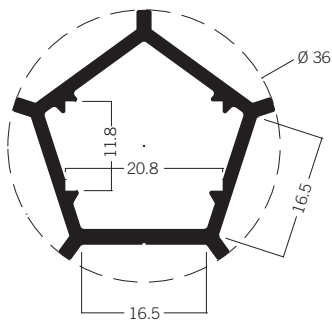
M 1980* Luminous elements extrusion 2.65 kg
