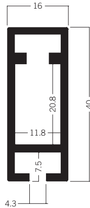
Z 4401* Beam extrusion 40 mm 3.38 kg
