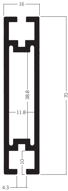
Z 110 Beam extrusion 70 mm 5.42 kg
