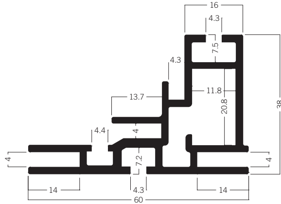
M 1910* Tension fabric extrusion for light frame 60 mm 7.62 kg
