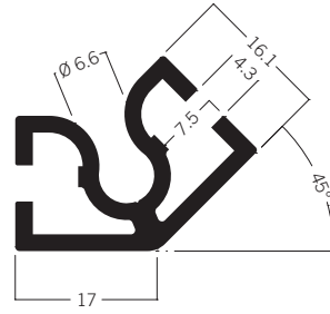
V 2020** Exterior corner extrusion 135° 2.63 kg
