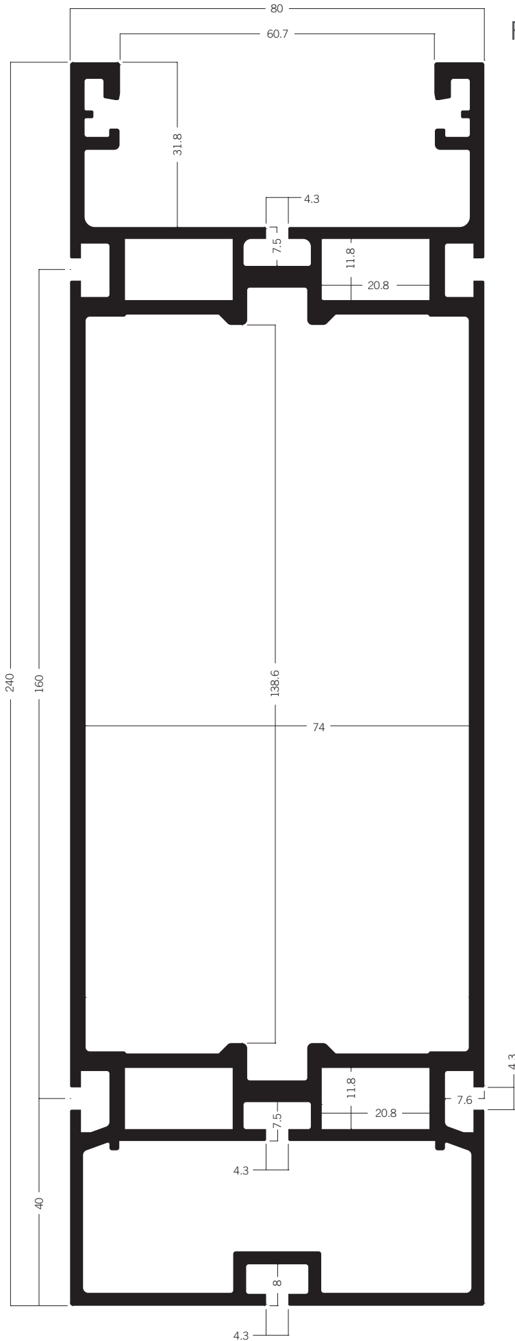
R 102 Rectangular extrusion 240 mm 53.23 kg
