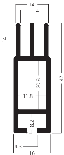
M 1504 Tension fabric extrusion, cube 4.57 kg
