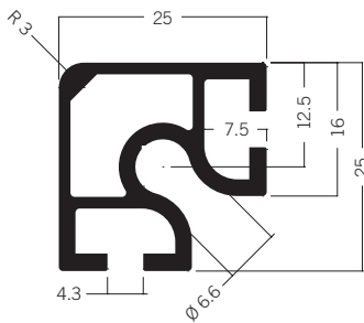
V 2000* Square extrusion 25 mm 2.89 kg
