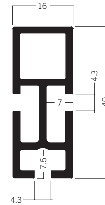
Z 4700* Rectangular extrusion 40 mm 3.49 kg
