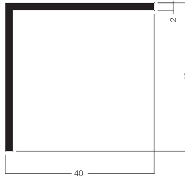
SO 400* Skirting extrusion OCTAeco floor 2.16 kg
