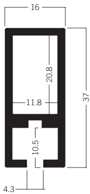
Z 310 Beam extrusion 37 mm 2.96 kg
