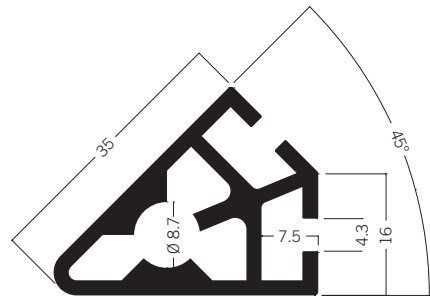
S 302 Upright extrusion 45° 4.03 kg
