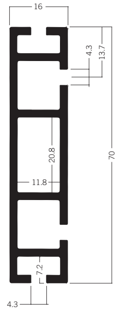
Z 164* Beam extrusion 70 mm 5.85 kg
