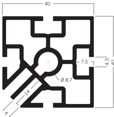
S 382 Upright extrusion 90°, with silicone edge groove
