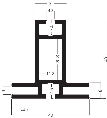
M 1307 Tension fabric extrusion 40 mm
