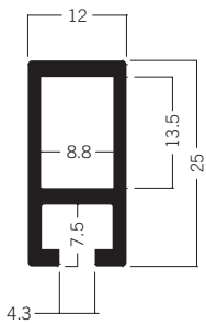
Z 305 Beam extrusion 25 mm 1.72 kg
