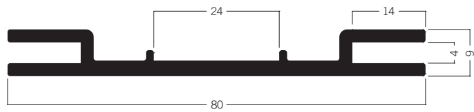
M 1325 Tension fabric extrusion 80 mm 5.33 kg
