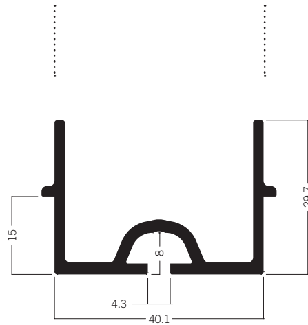
M 1155* Cover extrusion for M 1059 3.46 kg
