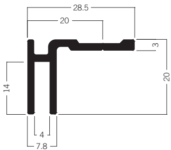
M 1322 Tension fabric extrusion 20 mm 2.03 kg
