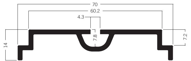
R 122* Cover extrusion 70 mm for R 102 2.88 kg
