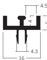
E 401 Lower track for sliding doors 0.45 kg
