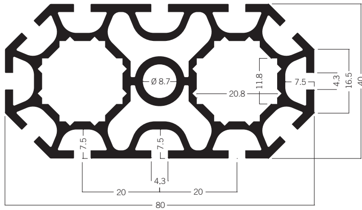
S 408 * Upright extrusion 80 mm 12.64 kg
