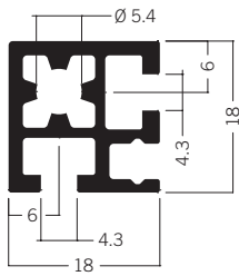
M 1618* Square extrusion 18 mm 1.99 kg
