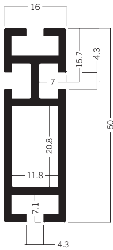
Z 460 Beam extrusion 50 mm 3.96 kg
