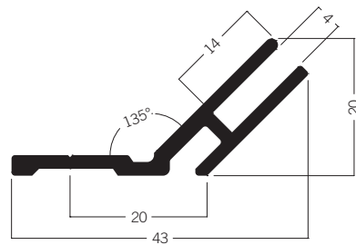
M 1321 Tension fabric extrusion 135° 2.29 kg
