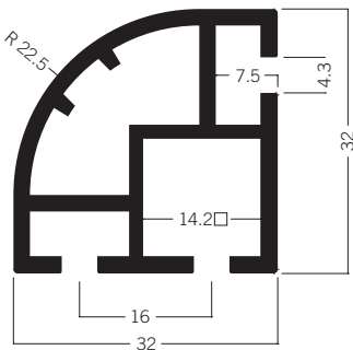
S 1105* Quarter-round extrusion 4.02 kg
