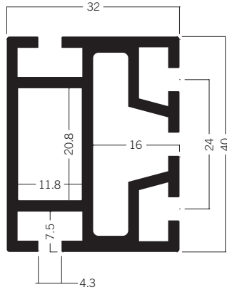
Z 2100 * Beam extrusion 40 mm 5.99 kg
