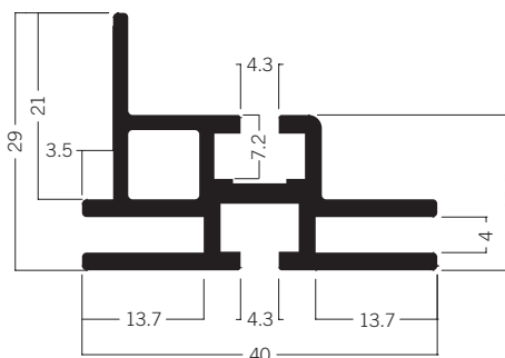
M 1970 Tension fabric extrusion for light frame 40 mm 4.34 kg
