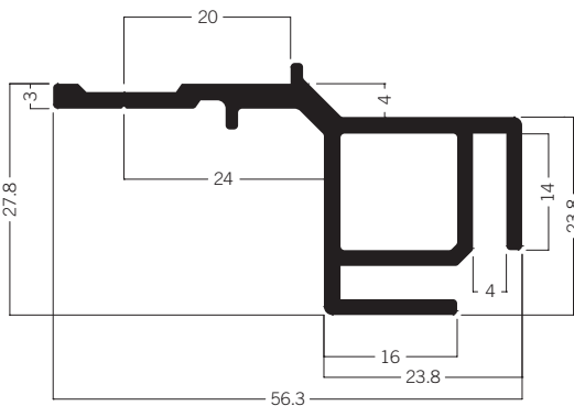
M 1322/I Tension fabric extrusion, internal corner 4.61 kg
