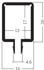
E 460 Cable retaining extrusion 0.73 kg
