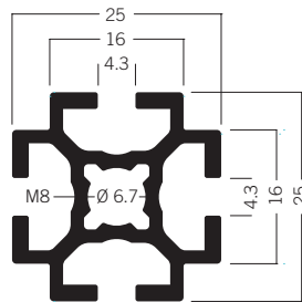
S 10* Square extrusion 25 mm 3.08 kg
