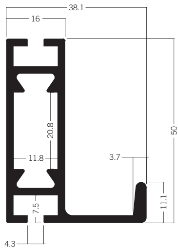
W 101* Beam extrusion 50 mm 5.56 kg
