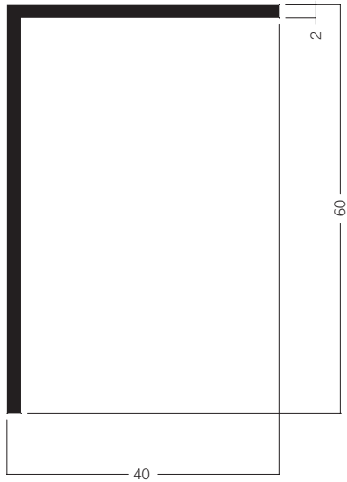
SO 500* Skirting extrusion 2.52 kg
