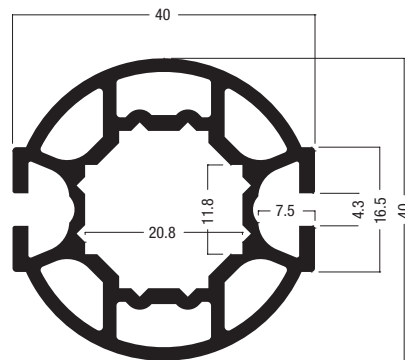
M 1202 Round extrusion 40 mm 6.10 kg
