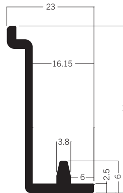
M 1581 Wall panel retainer, bottom 2.02 kg
