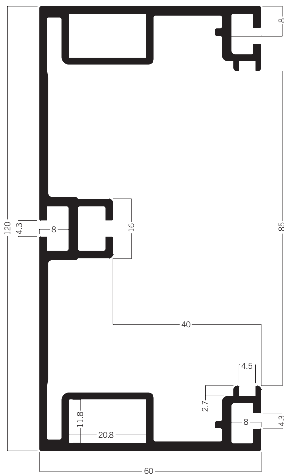
M 1060** Rectangular extrusion open 120 × 60 mm 5.61 kg
