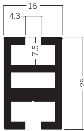
M 1602* Beam extrusion 25 mm 2.72 kg
