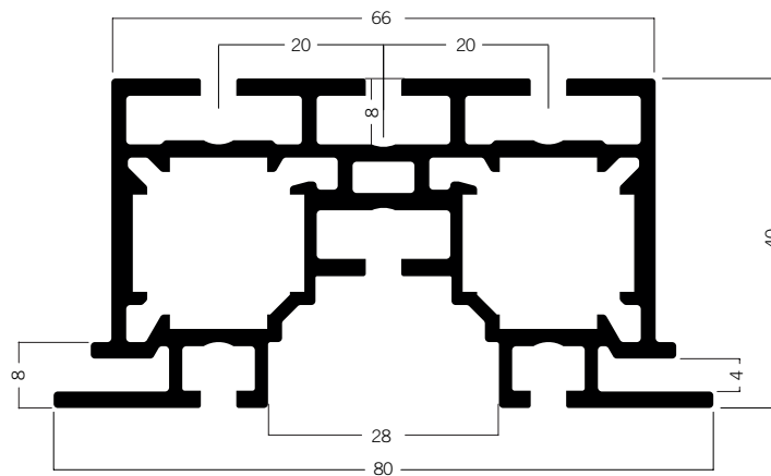
WP 860* Tension fabric extrusion 80 mm 12.99 kg
