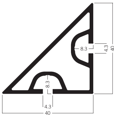
M 1072* Triangular extrusion 40 mm 4.85 kg
