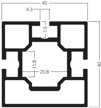
M 1005 Square extrusion 40 mm 6.66 kg
