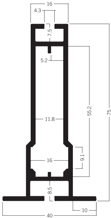
W 901* Frame extrusion 40 mm Panel 7.51 kg
