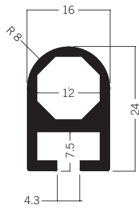
S 251* Hinged extrusion 24 mm 2.24 kg
