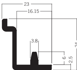
M 1571 Wall panel retainer, bottom 1.62 kg
