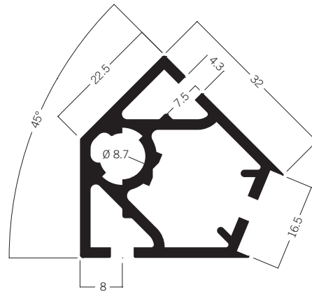
S 1129* Exterior corner extrusion 135° 4.74 kg
