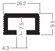
W 416* Insert extrusion 16 mm 1.05 kg
