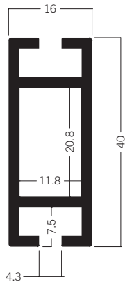
Z 4400 Beam extrusion 40 mm 3.20 kg
