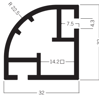
S 1100* Quarter-round extrusion 4.06 kg
