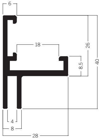
M 1302* Tension fabric extrusion 40 mm 3.49 kg
