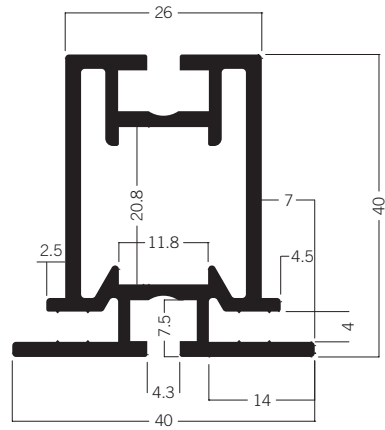
W 906 Tension fabric extrusion 40 mm
