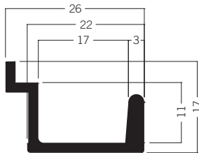
W 110* Adaptor extrusion for cladded wall 1.47 kg
