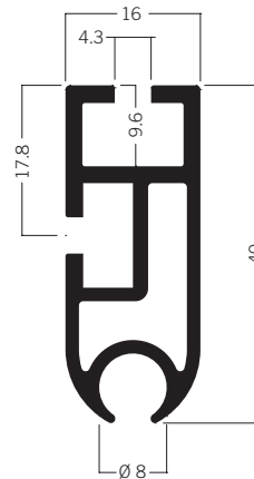
M 1356 Fabric suspension extrusion 40 mm 3.20 kg
