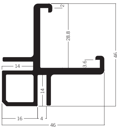
M 1332 Tension fabric extrusion, cube 5.94 kg
