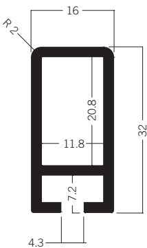
Z 303 Beam extrusion 32 mm 2.70 kg
