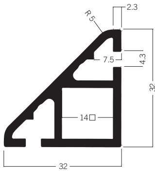
S 1302* Triangular extrusion 32 mm 3.20 kg
