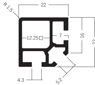
M 1625** Square extrusion 22 mm 2.15 kg
