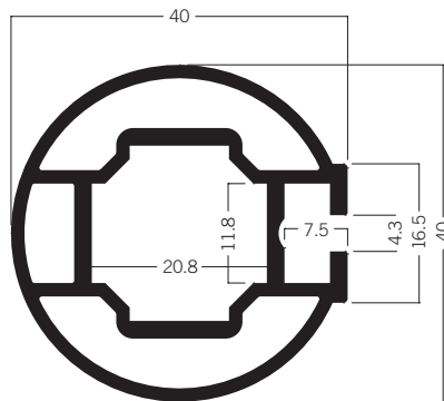
M 1201* Round extrusion 40 mm 5.25 kg
