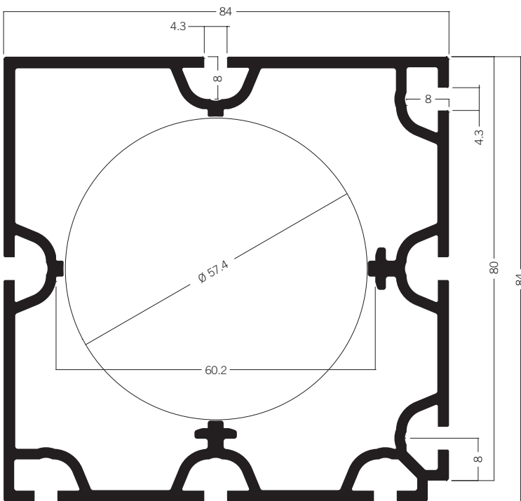
DFS 84/6000* Upright extrusion 80 mm 46.28 kg
