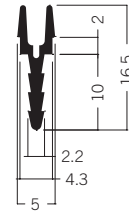
E 452* Extrusion connector 0.23 kg
