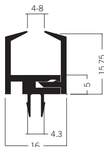
E 420 Glass panel retainer 0.83 kg
