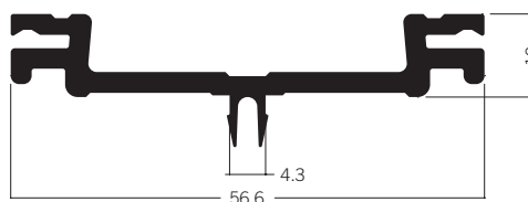
C 159* Adaptor extrusion 10 × 57 mm 2.04 kg
