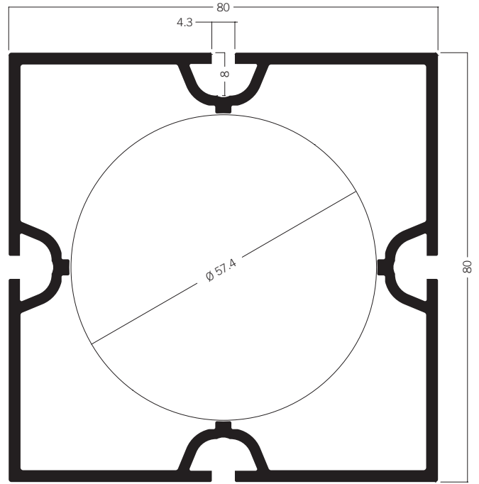
M 1020 Square extrusion 80 mm 11.51 kg
