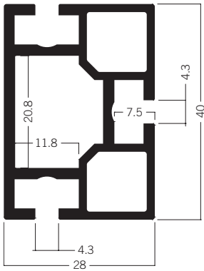
M 1069 * Rectangular extrusion 40 mm 5.71 kg
