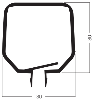
E 463 Cable retaining extrusion 1.20 kg
