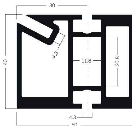
CO 730** Tension fabric extrusion 11.75 kg
