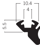
E 445* Anti-rattle strip 3.50 kg
