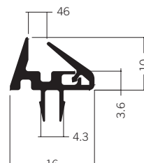
E 424 Glass panel retainer 0.45 kg
