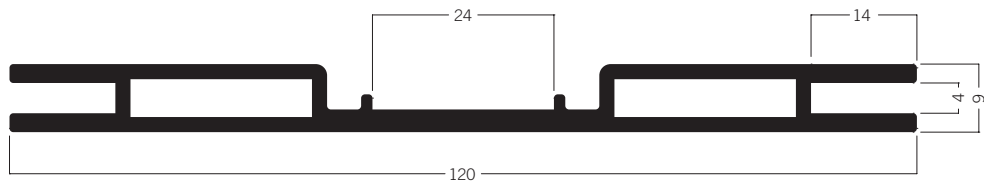
M 1330 Tension fabric extrusion 120 mm 8.28 kg
