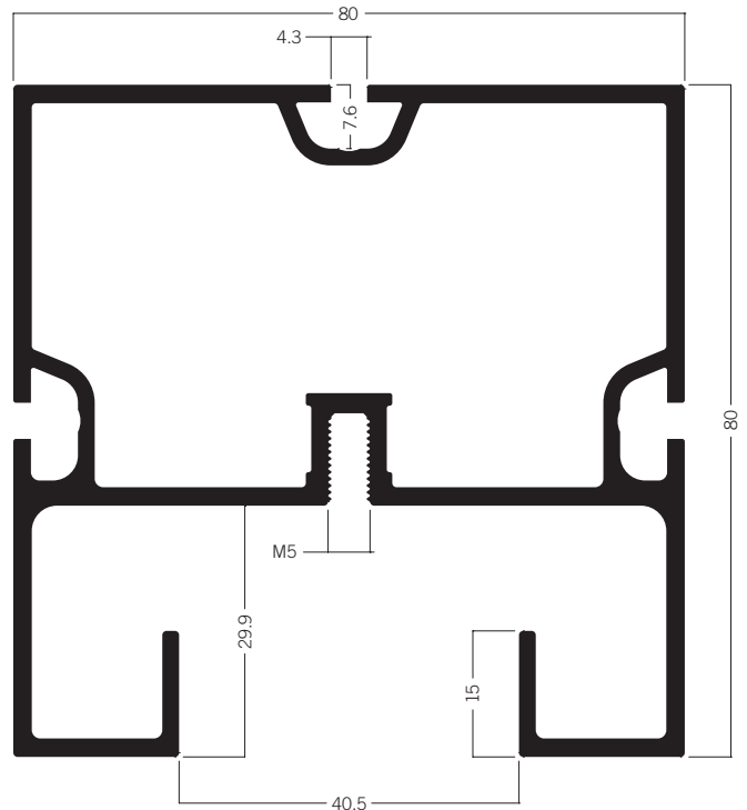
M 1059* Light track mounting extrusion 80 mm 15.92 kg
