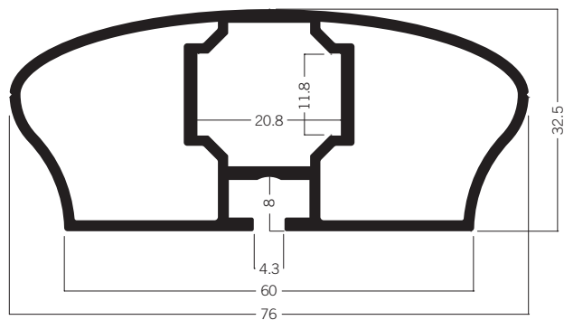
DFL 400A* Handrail extrusion 7.12 kg
