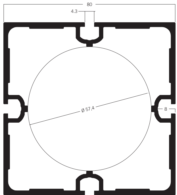
U 1020 * Square extrusion 80 mm 15.50 kg
