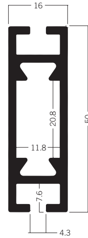
Z 408* Beam extrusion 50 mm 4.39 kg
