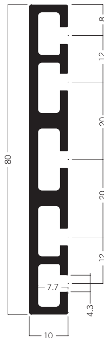
M 1063* Connecting extrusion 80 mm 5.46 kg
