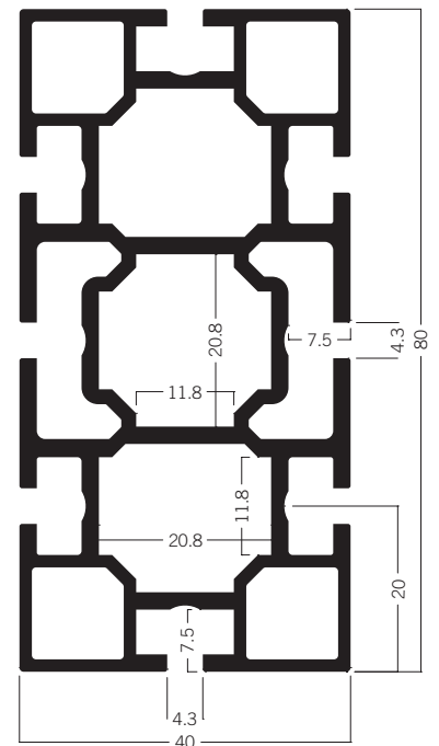
M 1092 * Rectangular extrusion 80 mm 14.60 kg
