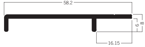
M 1572 Wall panel retainer, top 1.77 kg
