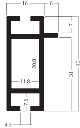
Z 4300* Beam extrusion 40 mm 3.54 kg
