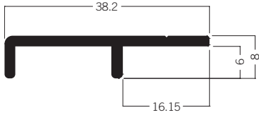
M 1562 Wall panel retainer, top 1.37 kg
