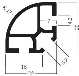
M 1620* Quarter-round extrusion 1.80 kg
