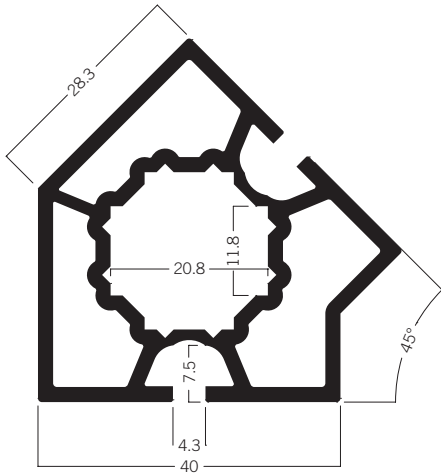
M 1009 Exterior corner extrusion 135° 7.82 kg
