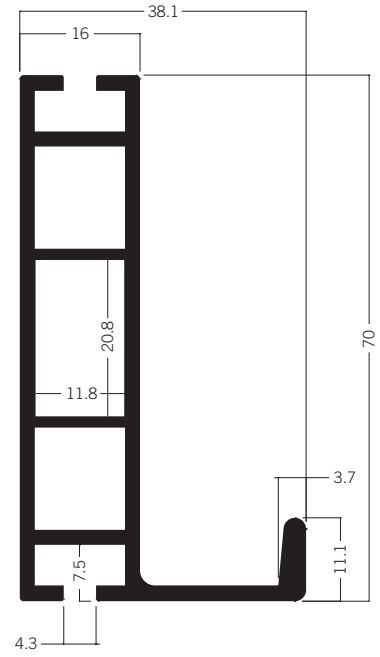
W 103* Beam extrusion 70 mm 6.51 kg
