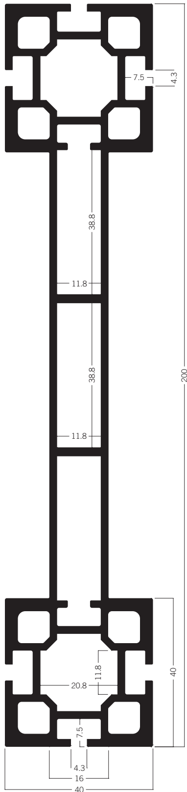
M 770 * Beam extrusion 200 mm 35.53 kg
