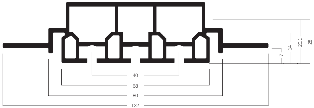
WP 820* T-connection extrusion 11.70 kg
