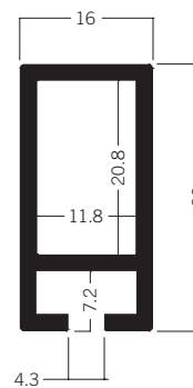
Z 308 Beam extrusion 32 mm 2.68 kg
