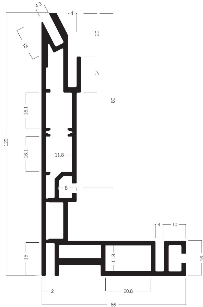
U 1060* Tension fabric extrusion 120 mm 16.20 kg
