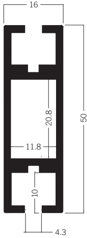
Z 400 Beam extrusion 50 mm 4.39 kg
