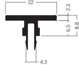
M 1846* Cover extrusion 0.51 kg
