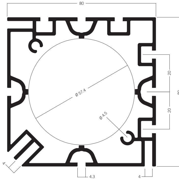
WP 850* Upright extrusion 90°, with silicone edge groove 16.48 kg
