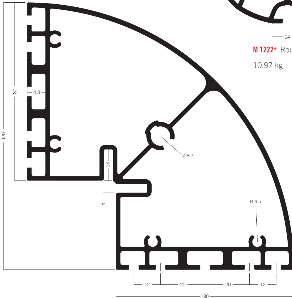
M 260* Upright extrusion 90° 25.50 kg
