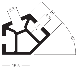
M 1629* Exterior corner extrusion 135° 2.15 kg
