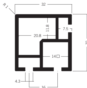
S 1125* Square extrusion 32 mm 4.03 kg
