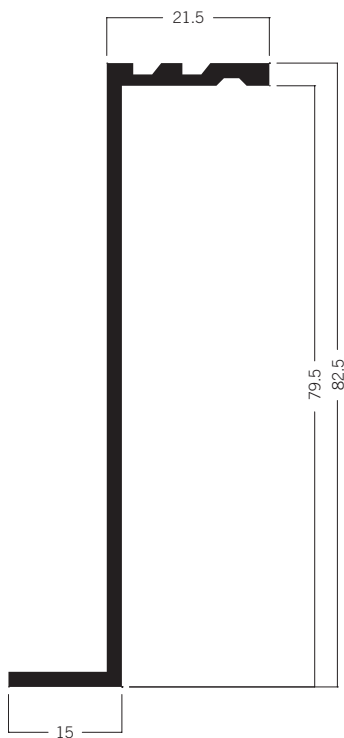
M 1520* Panel retainer extrusion for 80 mm system 3.85 kg
