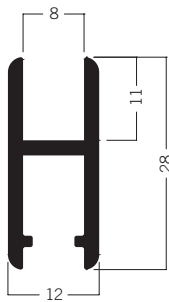
E 472* Runner frame extrusion 1.74 kg
