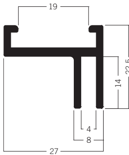
M 1309 Tension fabric extrusion 22.5 mm 2.53 kg
