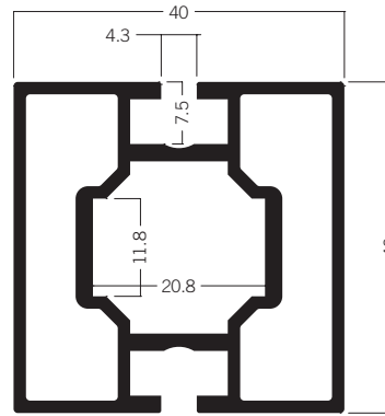
M 1002 Square extrusion 40 mm 5.55 kg
