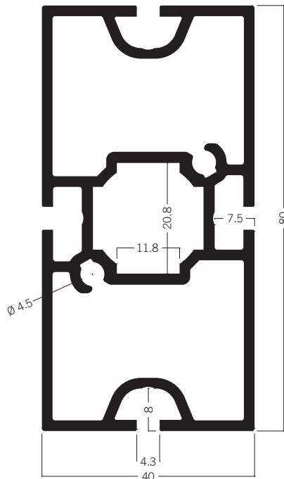
M 1025 Rectangular extrusion 80 mm 10.22 kg
