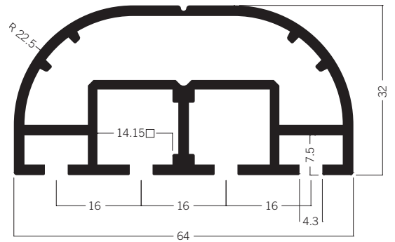
S 1106* Semi-circular extrusion 6.98 kg
