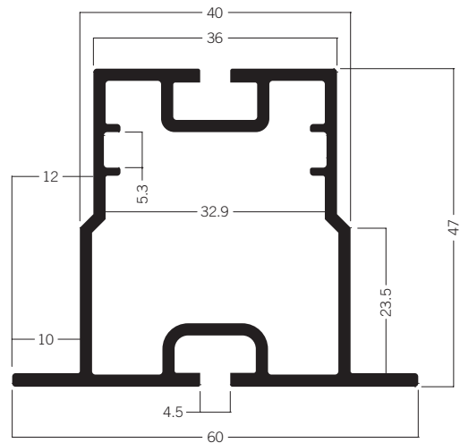
W 825* Frame extrusion 60 mm Panel (USA) 7.20 kg
