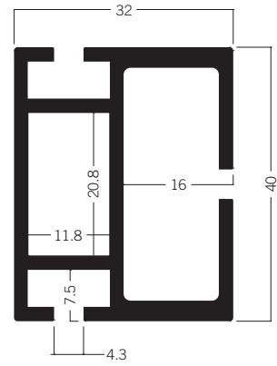
Z 2105 * Beam extrusion 40 mm 5.56 kg
