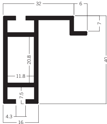
Z 4100* Beam extrusion 40 mm 4.14 kg
