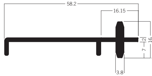
M 1577 Wall panel retainer, center 2.45 kg
