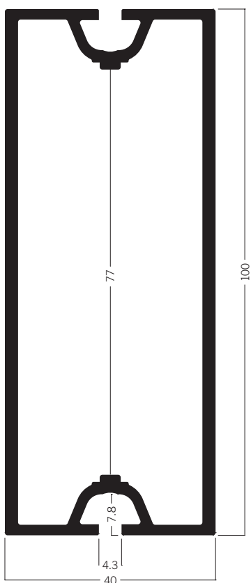
M 1029* Rectangular extrusion 100 mm 11.88 kg
